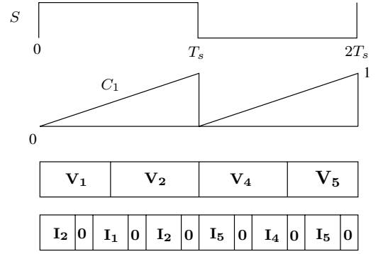
Fig. 5. Flux balance
