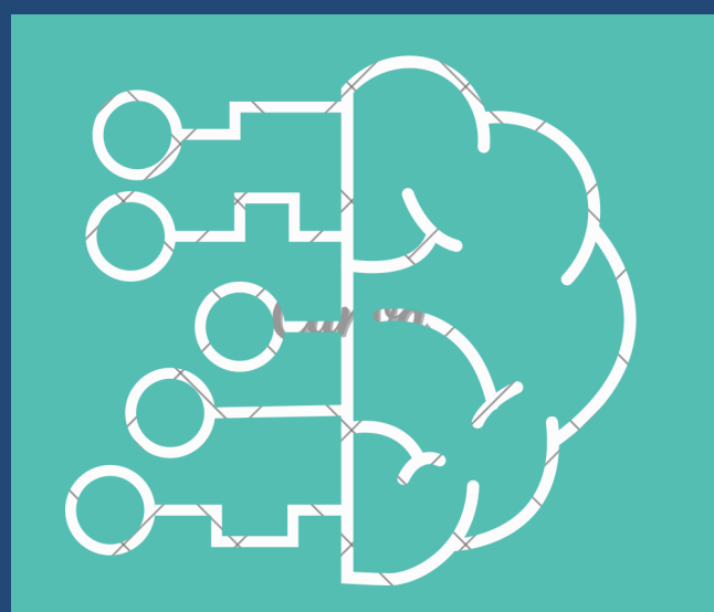
Machine Learning
